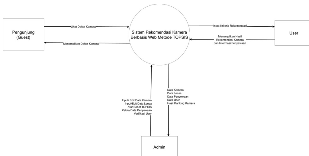
Gambar 4. 7 Data Flow Diagram (DFD)
