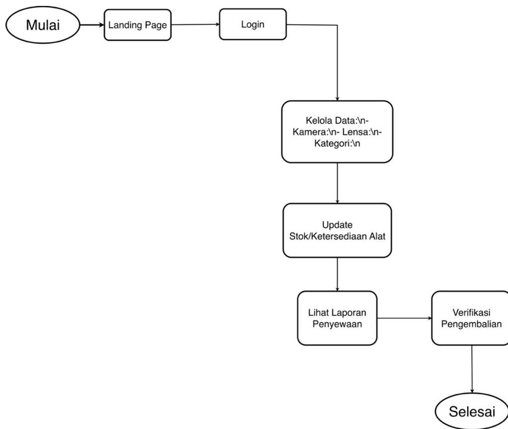
Gambar 4. 5 Flowchart Admin
