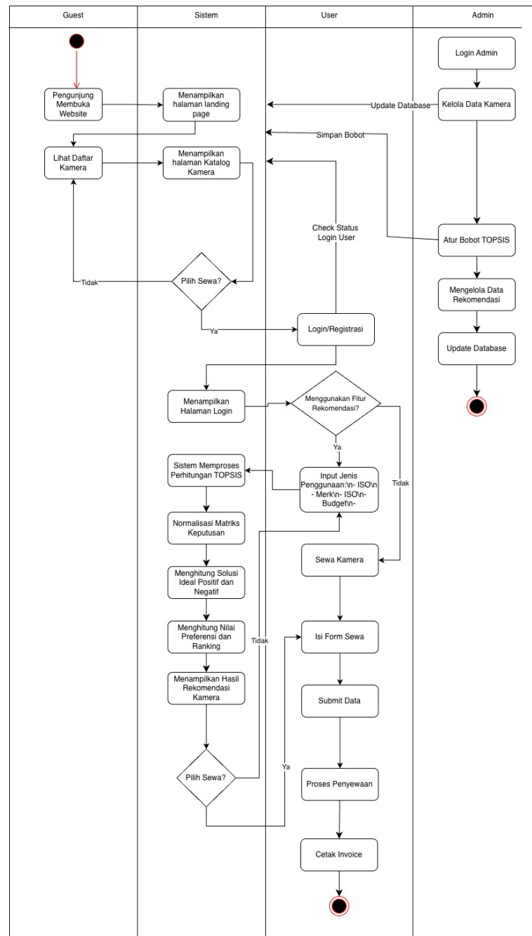
Gambar 4. 6 Activity Diagram
