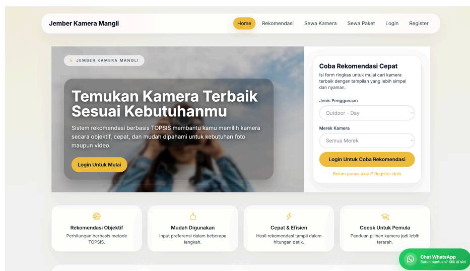
Gambar 4. 20 Landing Page
