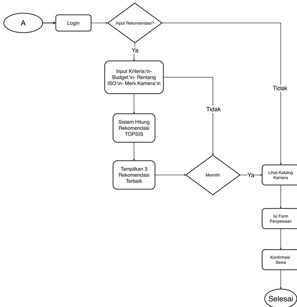
Gambar 4. 4 Flowchart User
