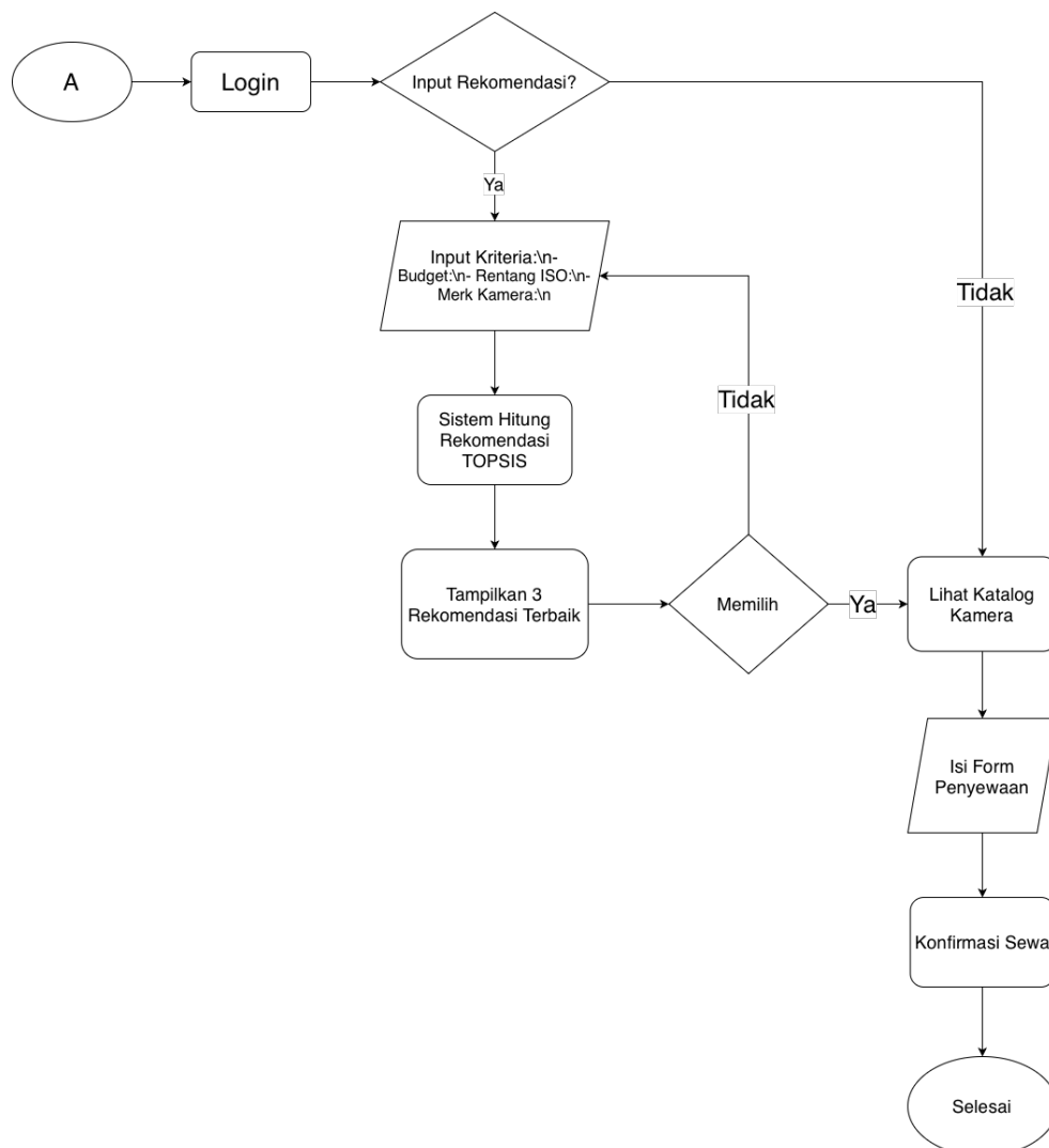
Gambar 4. 4 Flowchart User
