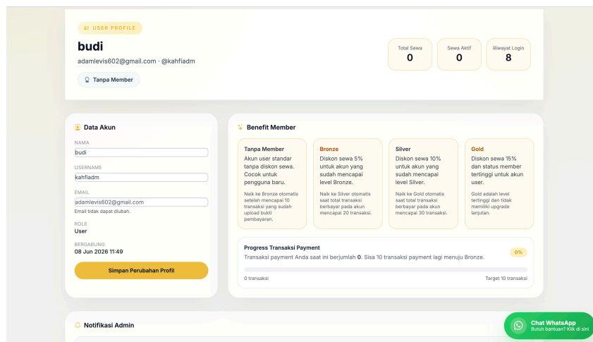
Gambar 4. 25 Dashboard User
