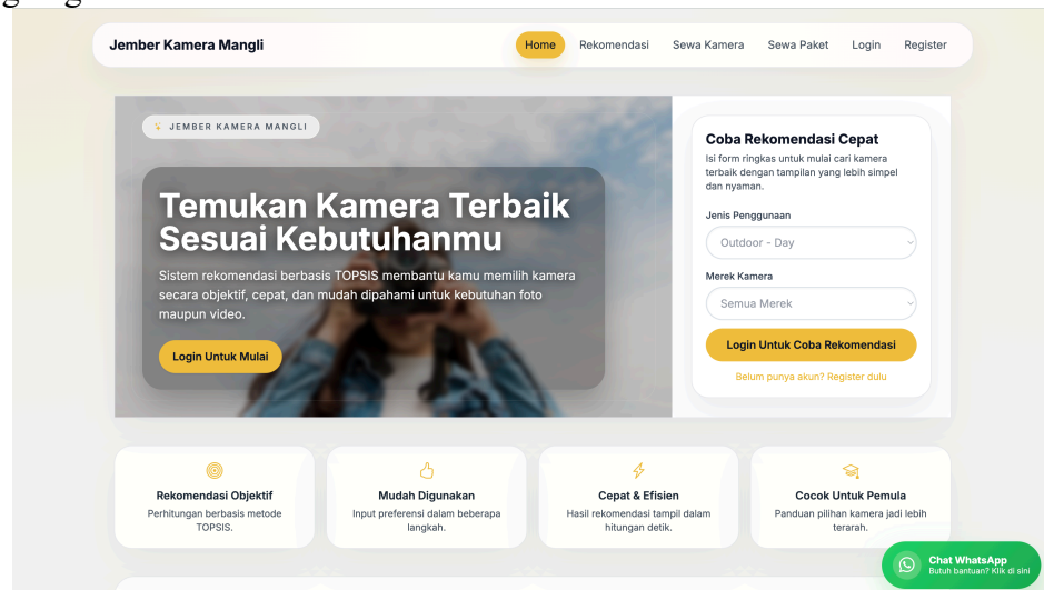
Gambar 4. 19 Landing Page
