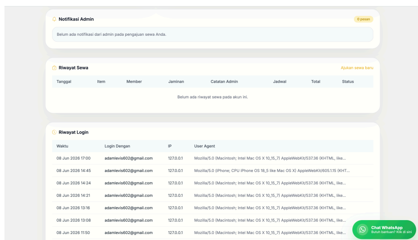
Gambar 4. 26 Dashboard User
